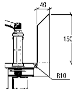
STANDARD BACKSPLASH
