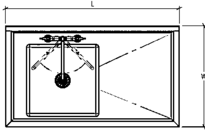
1 COMPARTMENT - L/R DRAIN BOARD
