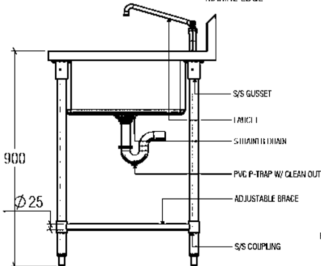
SINGLE & TWO COMPARTMENT SINK SECTION
