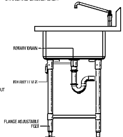
3 COMPARTMENT SINK SECTION
