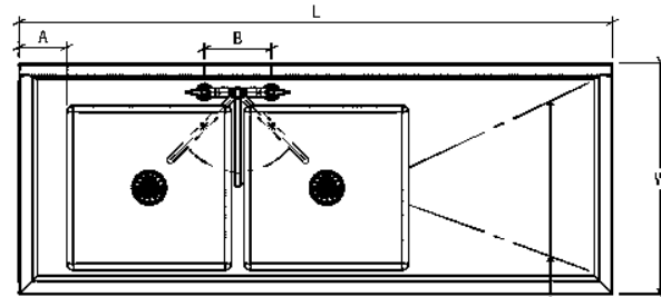
2 COMPARTMENTS - L/R DRAIN BOARD
