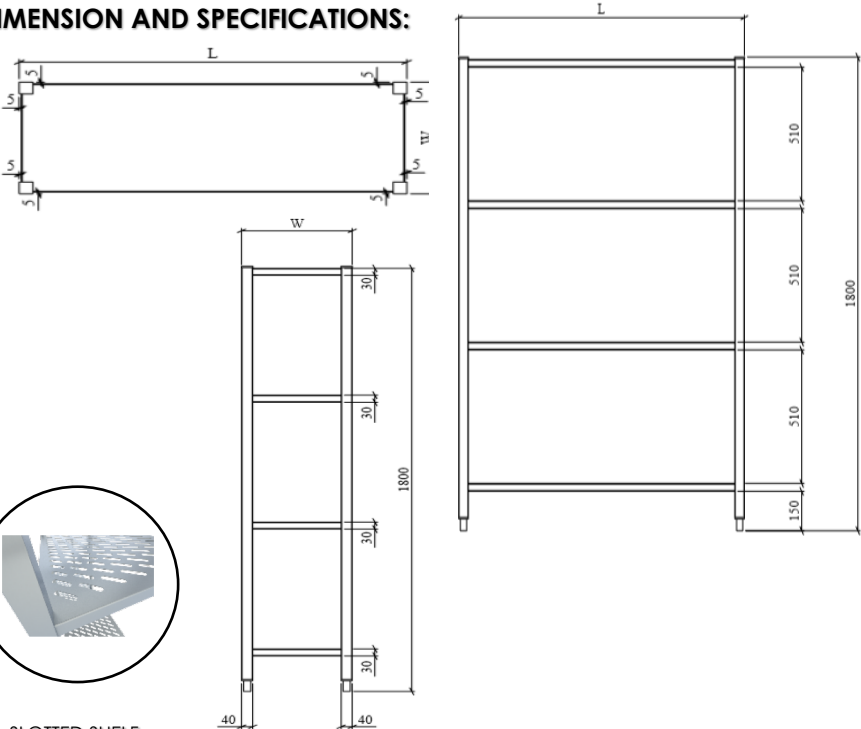
SLOTTED SHELF DETAIL
