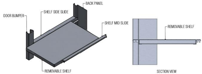
REMOVABLE SHELF ASSEMBLY
