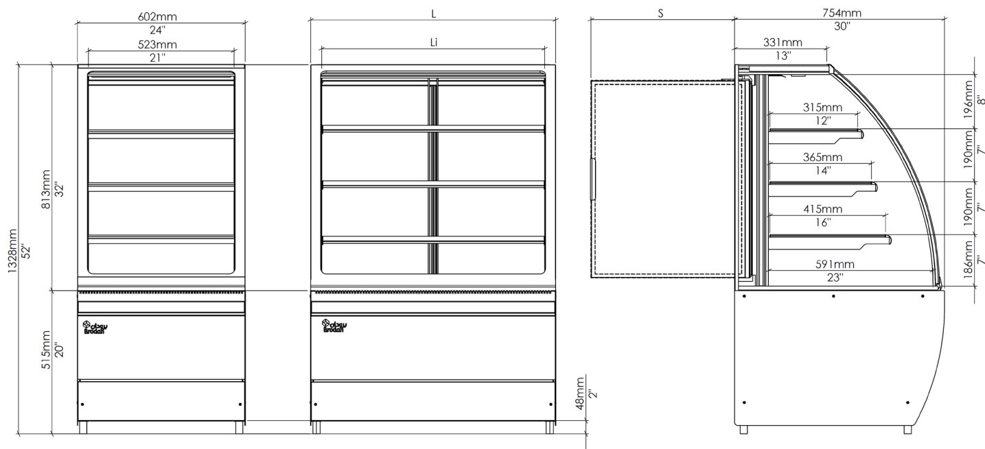
600 Front Elevation
